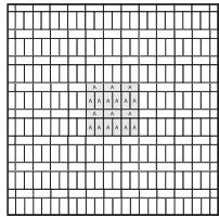
Stack Bond (Variant) A Units
