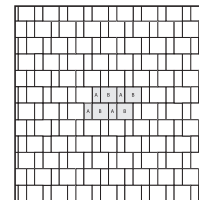
A, B & C Units Pattern #12 A-33% B-67%
