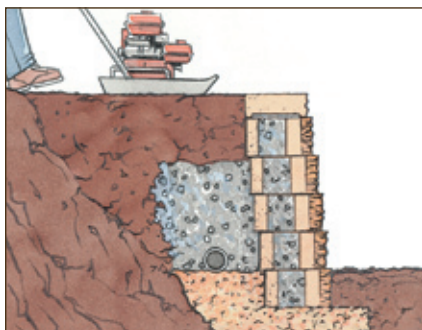
Diagram 8—Compaction
